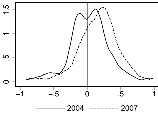
(c) Imputed Cost, no covariates
