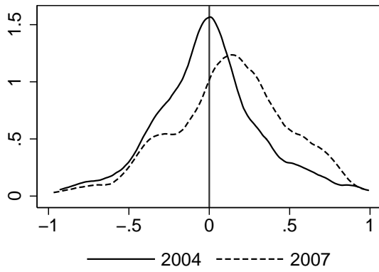
(a) Net price, no covariates
