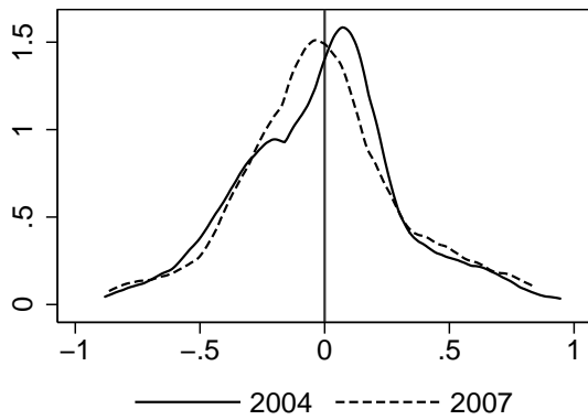
(e) Mark up, no covariates
