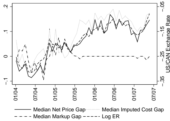
(a) Net, all stores
